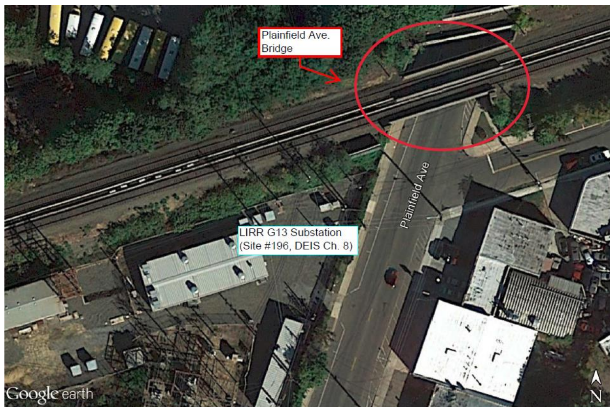
Figure 3.3 – Plainfield Avenue Bridge
